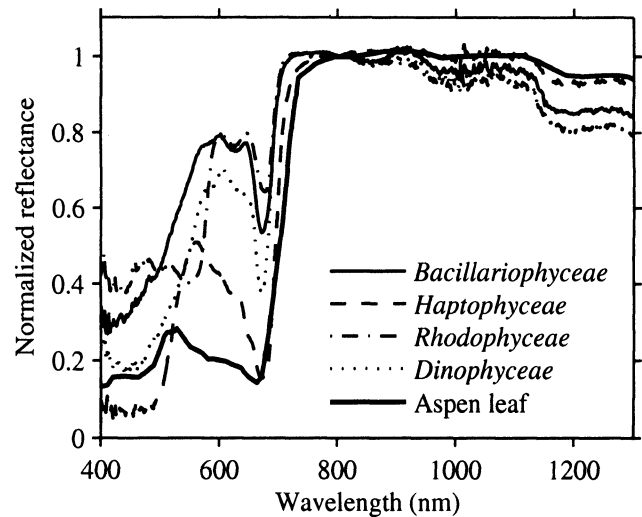
Fig. 7. Relative reflectance of unicellular algal cultures captured onto GF/F filters increases strongly from 680 to 710 nm, producing a red edge typical of photosynthetic tissues. The reflectance spectrum from a terrestrial aspen leaf (Hall et al. 1991) is shown for comparison. Spectra are normalized to reflectance at 800 nm and do not contain a solar-stimulated fluorescence peak centered at 683 nm.
