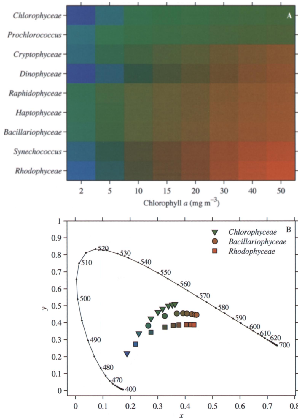
Fig. 5. (A) Color of the sea surface as a function of surface biomass concentration (Chl a used as a proxy) for different phytoplankton taxa. Color was modeled from water-leaving radiance using the CIE color matching functions and mean absorption and backscattering properties for each taxa. (B) The chromaticity coordinates for a selection of three algal taxa are shown on a CIE chromaticity diagram (Kelly 1943) as Chl a increases from 2 \text{mg m}^{-3} (lower left points) to 50 \text{mg m}^{-3} (upper right points). For clarity, the color of each symbol corresponds to the color presented for that algal group in panel (A).
