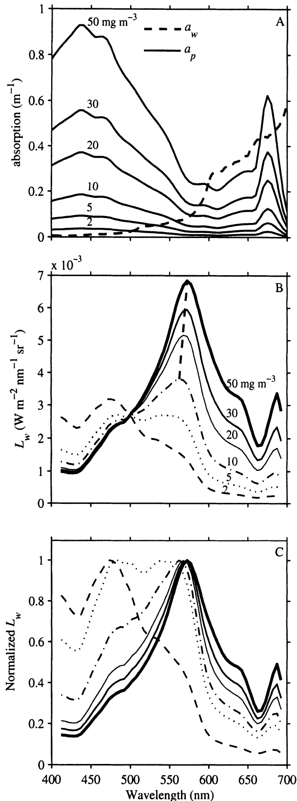
Fig. 4. (A) Particulate absorption coefficient for a diatom showing the increase in absorption with increasing concentration. The wavelength at which absorption due to phytoplankton and that due to pure water (Pope and Fry 1997) intersect represents the minimum in absorption and the maximum or peak reflectance. (B) Spectral variability in water-leaving radiance ( L_w ) modeled for
